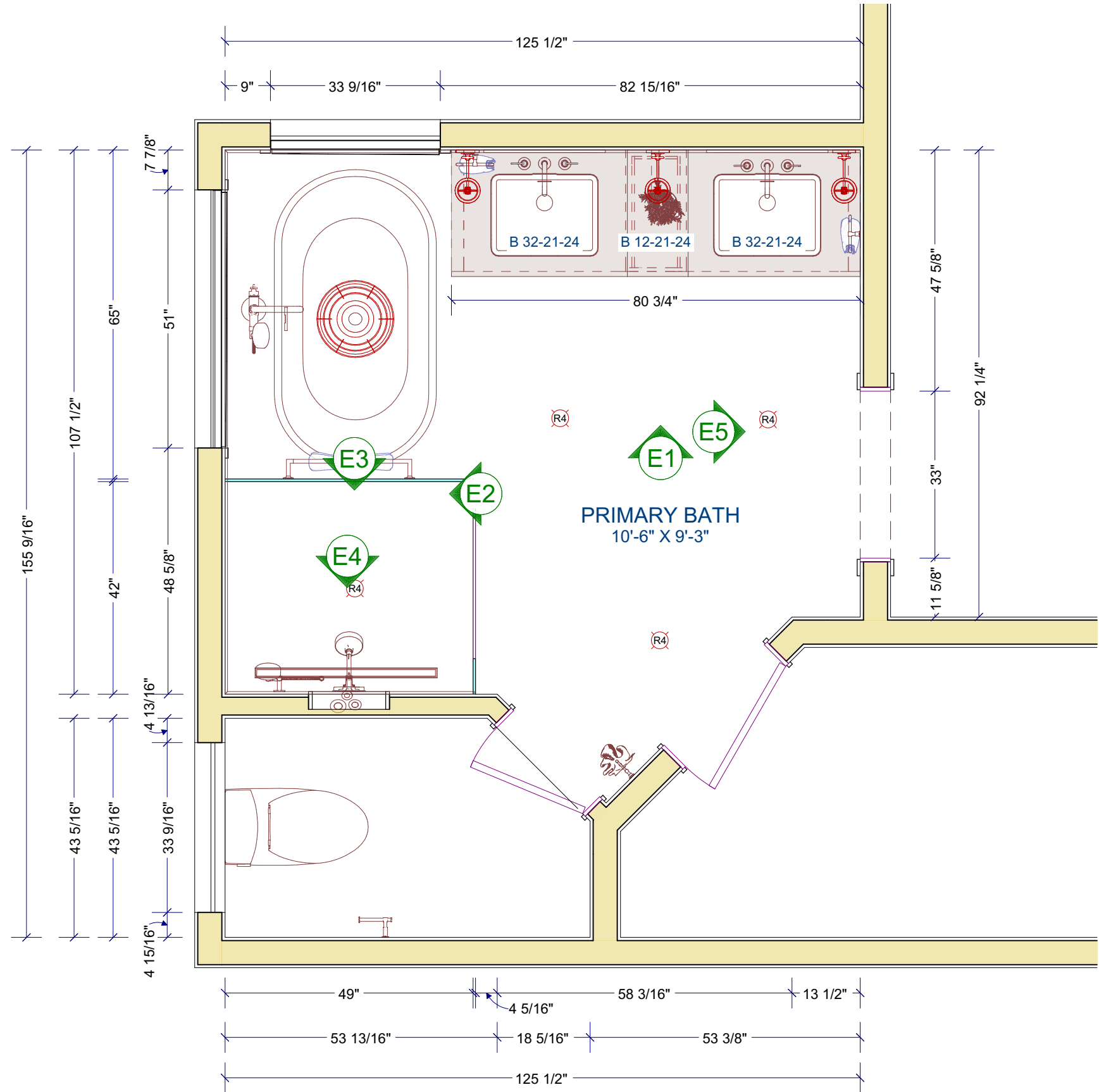
PLAN VIEW 1/2 in = 1 ft
