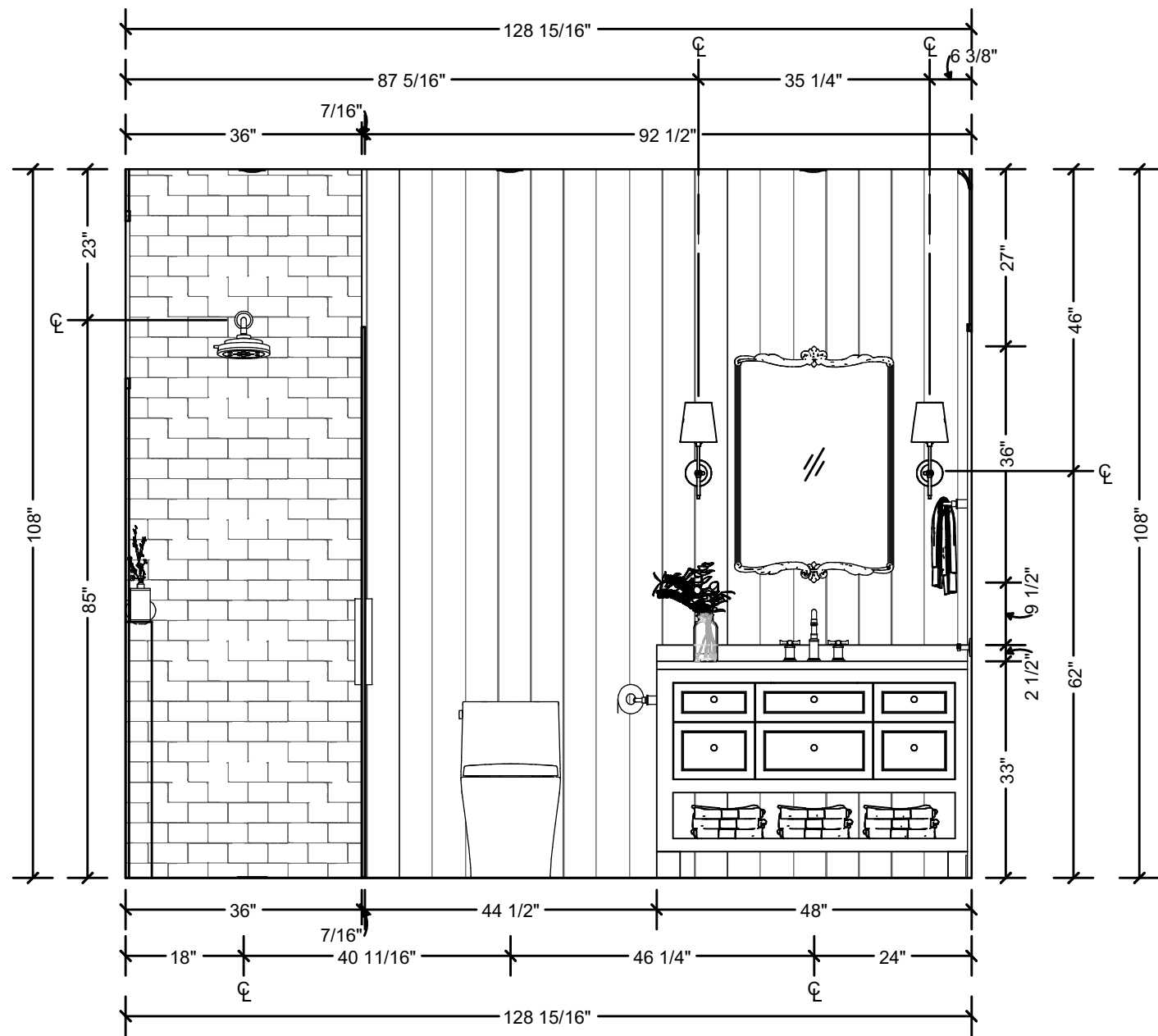
Guest Bath Elevation 1 1/2 in = 1 ft
