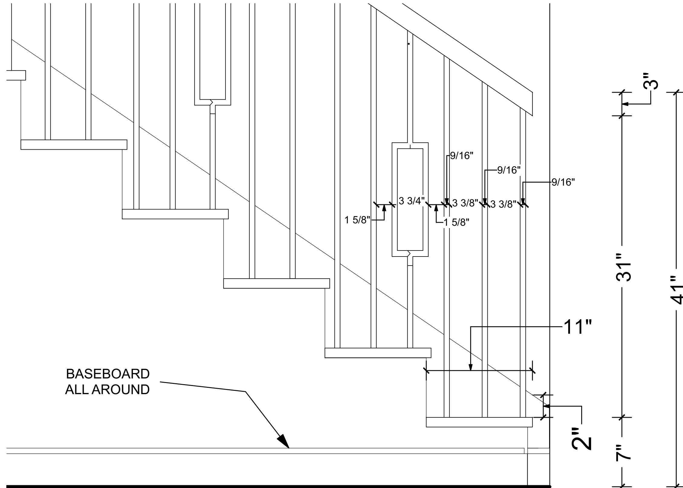
Stairs Elevation 1 2 in = 1 ft
